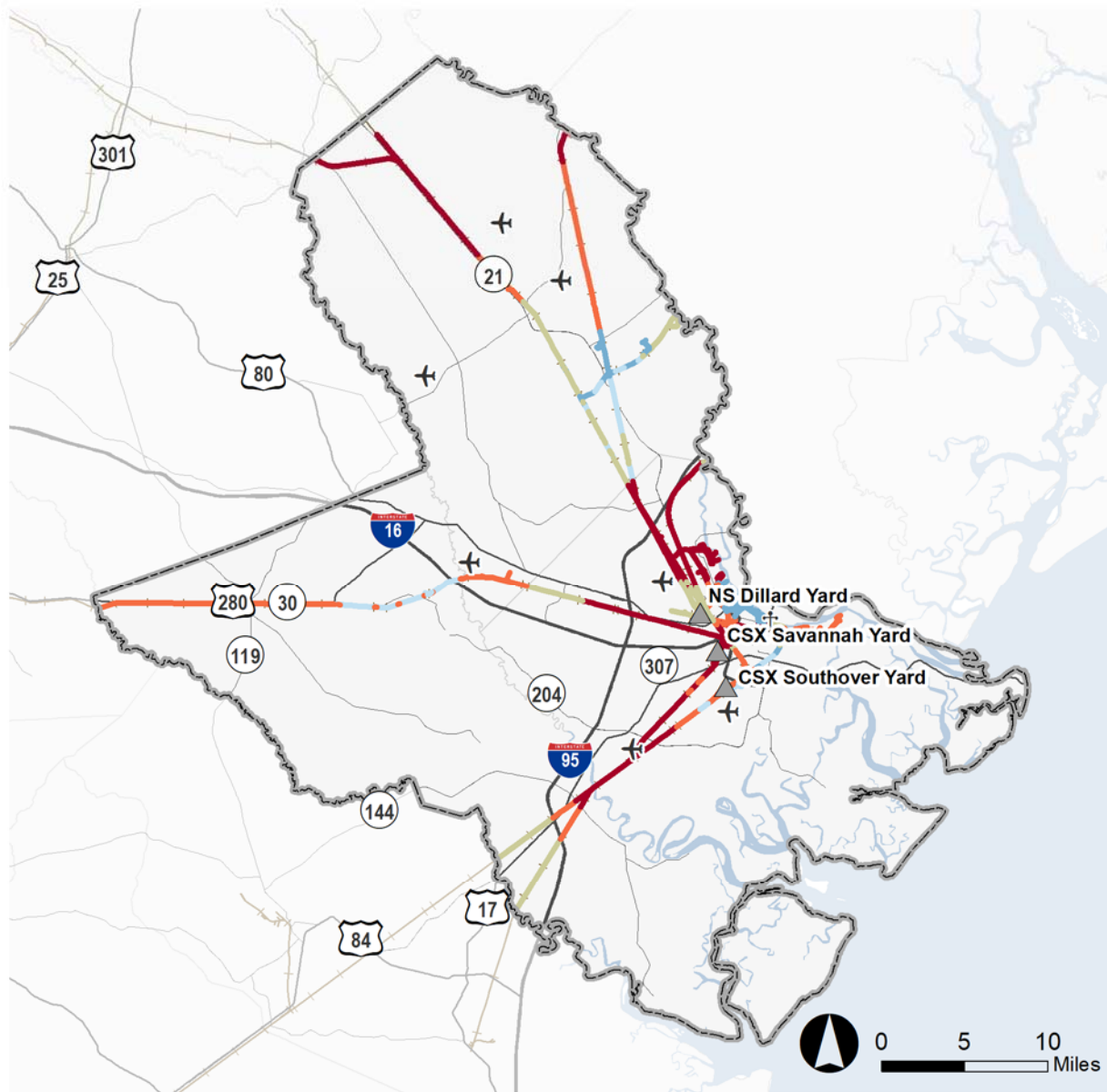
FIGURE 2.13 VULNERABLE RAILROAD ASSETS
