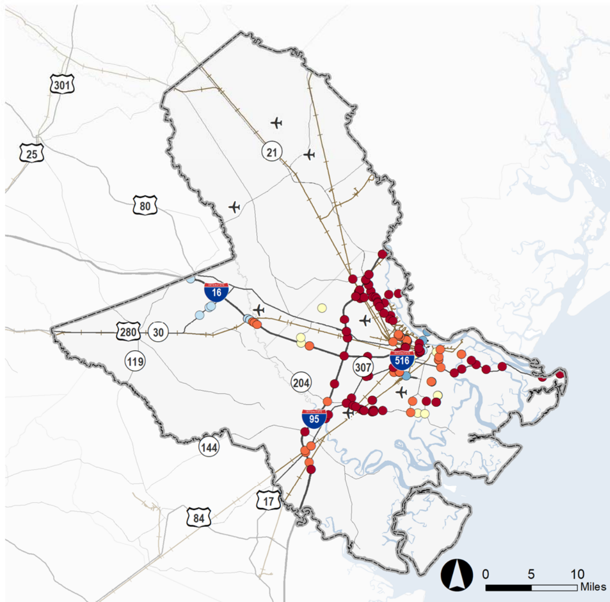
FIGURE 2.12 VULNERABLE BRIDGE ASSETS
