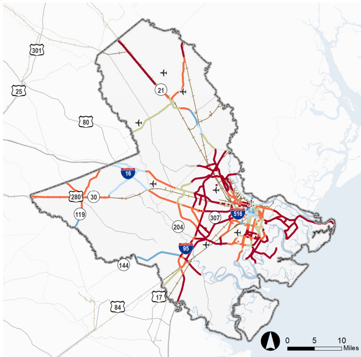
FIGURE 2.11 VULNERABLE HIGHWAY ASSETS
